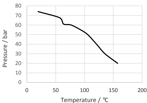
BURST PRESSURE
