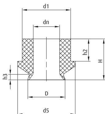
With straight passage – Series SV-TG
