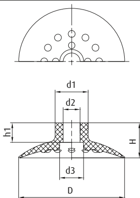
Flat vacuum cups – Series SV-VUF Ø 50 mm
