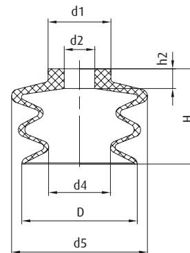
Bellows vacuum cups, 2.5 bellows – Series SV-VUB2 Ø 34 mm
