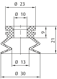
Bellows vacuum cups, 1.5 bellows – Series SV-SB1 Ø 30 mm
