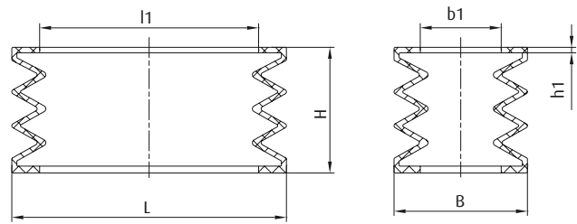
Bellows vacuum cups, 2.5 bellows, with flat sealing lip 52x25 | 60x29 mm
