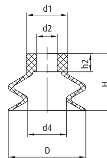
Bellows vacuum cups, 1.5 bellows – Series SV-VUB1 Ø 20 | 30 mm
