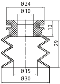
Bellows vacuum cups, 2.5 bellows – Series SV-SB2 Ø 30 mm
