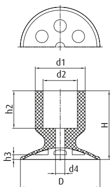
Flat vacuum cups – Series SV-VUF (pipe mounting) Ø 17 | 26 | 30 mm
