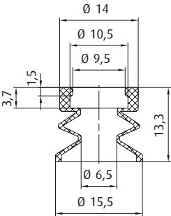
Bellows vacuum cups, 1.5 bellows – Series SV-SB1 Ø 15,5 mm
