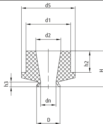
With conical passage – Series SV-TK
