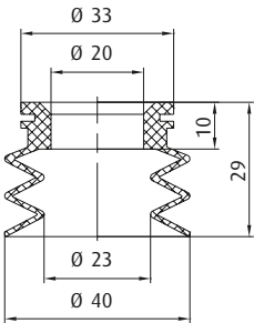
Bellows vacuum cups, 2.5 bellows – Series SV-SB2 Ø 40 mm
