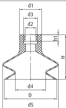
Bellows vacuum cups, 1.5 bellows – Series SV-VUB1 Ø 49 mm
