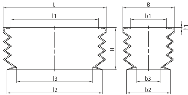
Bellows vacuum cups, 3.5 bellows, with thinly tapering, flexible sealing lip 80x30 | 80x40 | 80x50 mm
