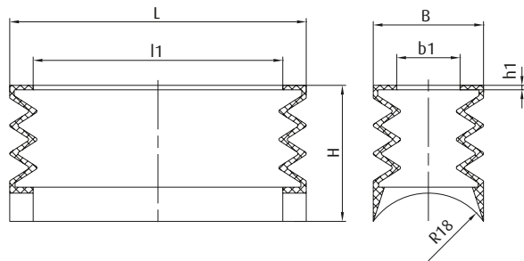
Bellows vacuum cups 2.5 bellows, for cylindrical products 79x29 mm
