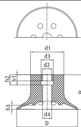
Flat vacuum cups – Series SV-VUF Ø 30 mm
